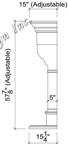
Side Elevation
