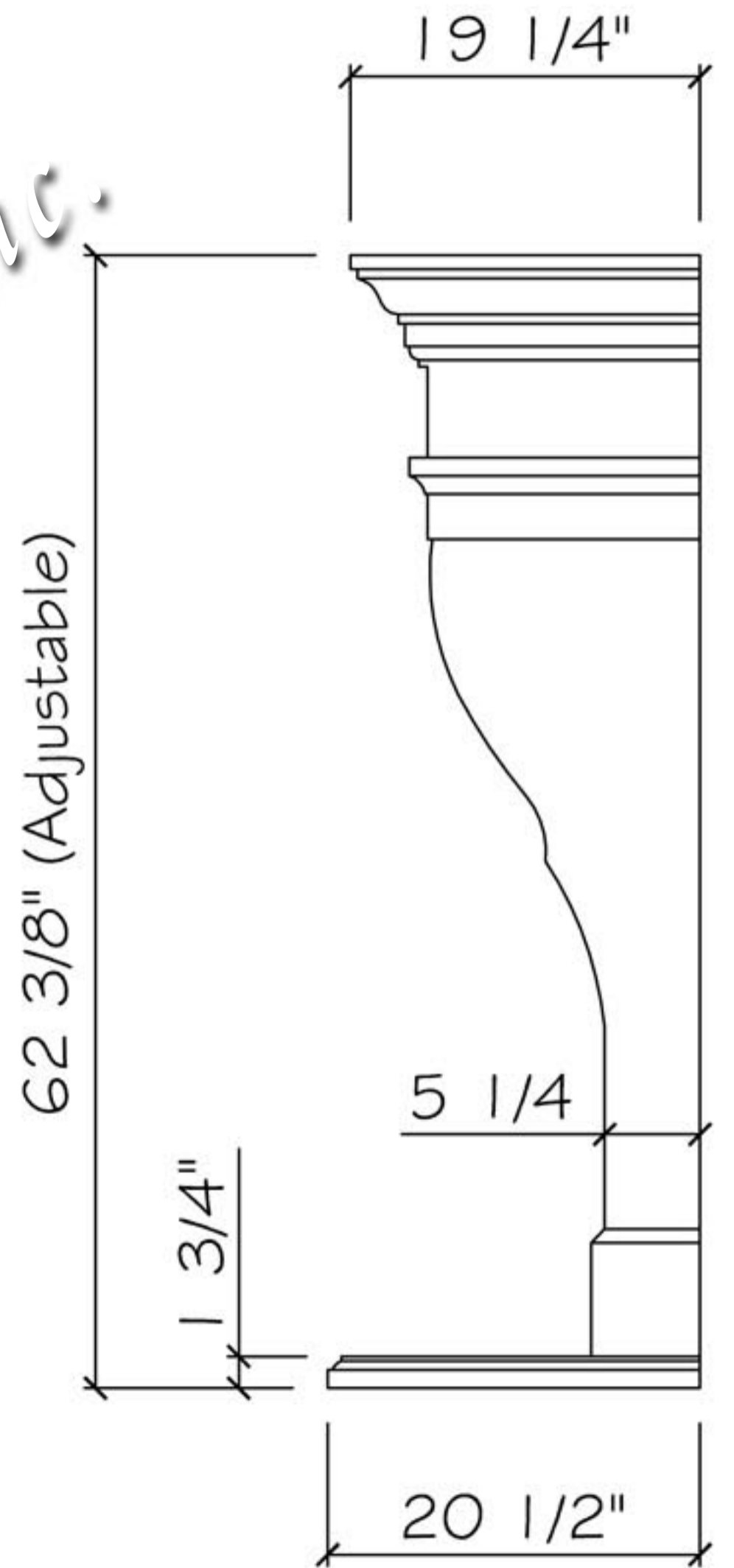
Side Elevation
