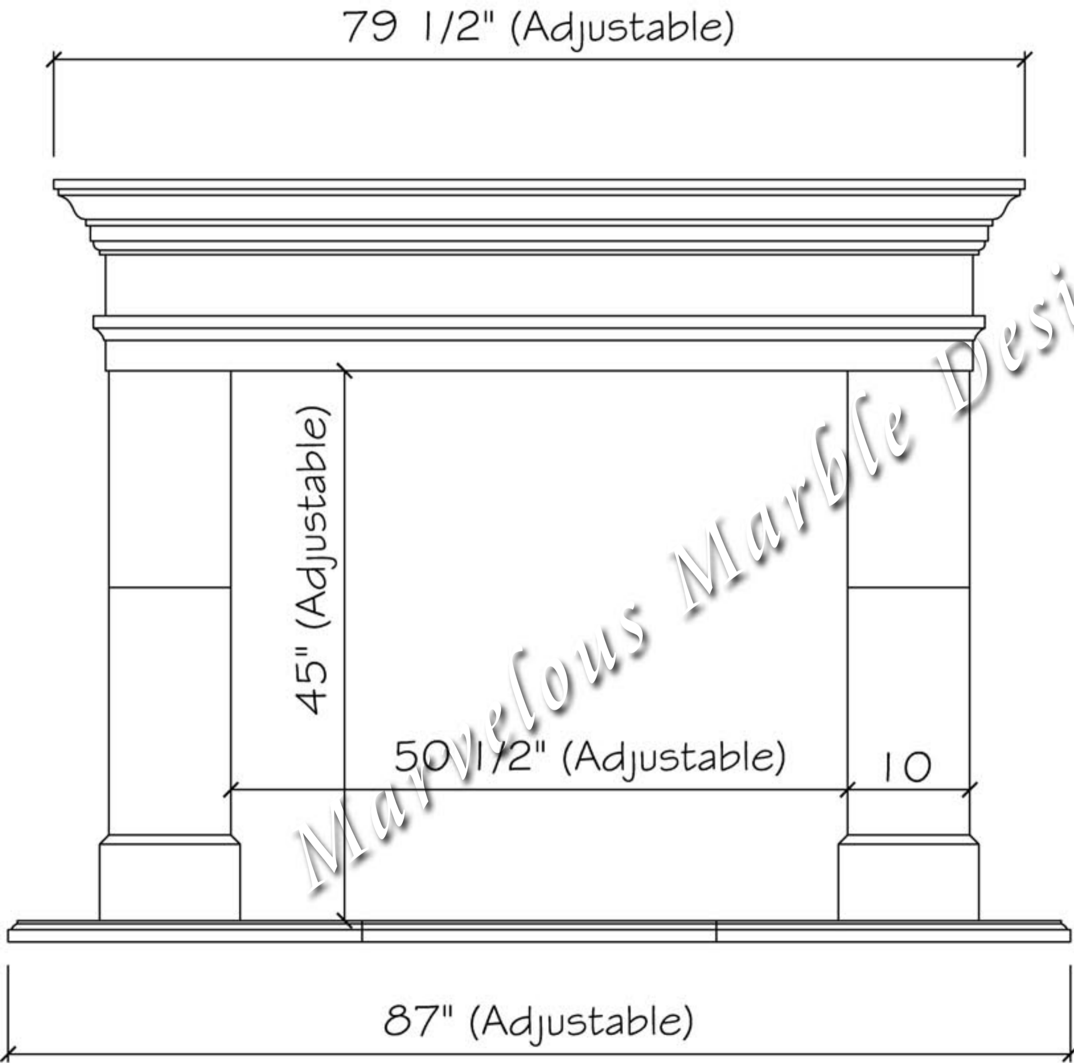
Front Elevation
